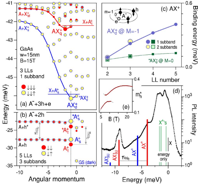
FIG. 5. (Color online) Calculated energy spectra of (a) 3h+e and (b) 2h systems in the presence of an ionized acceptor A^- in the middle of a symmetric quantum well. In (a), A^-X^+ pair states are connected with the solid lines, and AX_d^+ at angular momentum M=-1 is the spin-doublet ground state of an A^- -bound trion. In (c), the AX_d^+ binding energy is compared to the weakly bound ^*AX_d^+ at M=0 as a function of the number of included LLs and subbands (lines are a guide for the eye). In (b), four lowest final states for the AX_d^+ \rightarrow A^+ recombination are marked at M=-1 . In (d), the corresponding four-peak AX_d^+ emission spectrum is overlaid with the experimental data of Fig. 2(a). In (e), the hole effective mass m_h^* is extracted from the splitting of the experimental shake-up line, equal to the hole cyclotron energy as shown in (b). All data are for a 15 nm GaAs quantum well and, except for (e), for magnetic field B=15 T.
