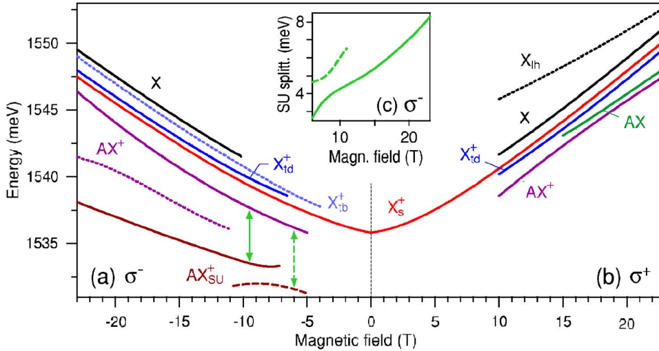
FIG. 3. (Color online) Magnetic field dependence of recombination energies identified in polarizations \sigma^- (a) and \sigma^+ (b) in the PL spectra in Fig. 2. (c) Splitting of the shake-up line.
