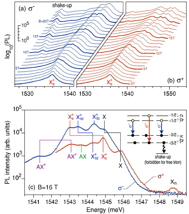
FIG. 2. (Color online) Top: Comparison of (a) \sigma^- and (b) \sigma^+ polarized PL spectra at a sequence of magnetic fields between B=0 and 23 T (same sample as in Fig. 1). Bottom: Magnified spectra at B=16 T. Several identified lines include free exciton X and three positive trions X^+ (spin-singlet and two spin-triplets), acceptor-bound exciton AX and trion AX^+ , and a light-hole exciton X_{lh} . Note different spin splittings of the X , AX^+ , and different X^+ states. Inset: Schematic of the \sigma^\pm polarized transitions of a positive spin-singlet trion.
