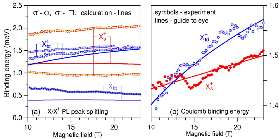
FIG. 4. (Color online) (a) Magnetic field dependence of the trion binding energies determined from the exciton-trion peak splittings, \Delta=E[X]-E[X^+] ; lines, numerical calculation of the corresponding Coulomb binding energies (i.e., binding energies ignoring the Zeeman term); (b) Coulomb binding energies of the singlet and dark triplet trions, obtained as \sigma^\pm averages \frac{1}{2}(\Delta^++\Delta^-) to remove Zeeman effect; lines, guide for the eye. The crossover occurs at B \approx 12 T, and adding the hole Zeeman term to E[X_s^+] shifts it to an even lower field. Note features around B=14.2 T, corresponding to \nu=\frac{1}{3} .
